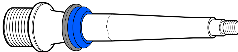
12. INSTALL THE OUTER SPINDLE SEAL FIRST, ROUNDED EDGE FACING AWAY FROM SMALL END OF THE SPINDLE. INSTALL THE INNER SEAL (DOUBLE-LIP SEAL) WITH THE POINTED END FACING TOWARD THE LARGE END OF THE SPINDLE.
